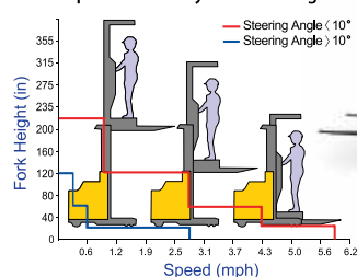
Travel Speed Control By Platform Height
